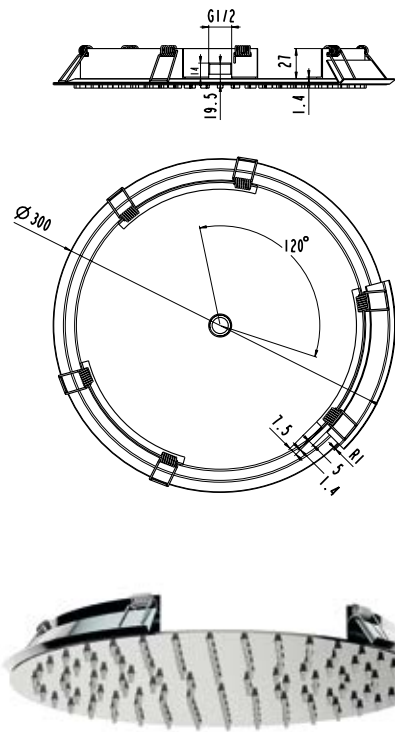
SHOWER HEAD ROUND Ø30 cm Material: Stainless Steel (SS304)
