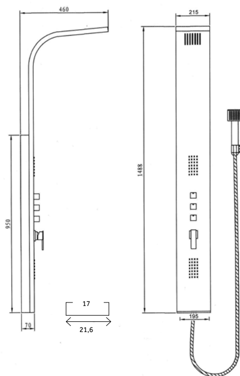
TECHNICAL DRAWING GOCTA
