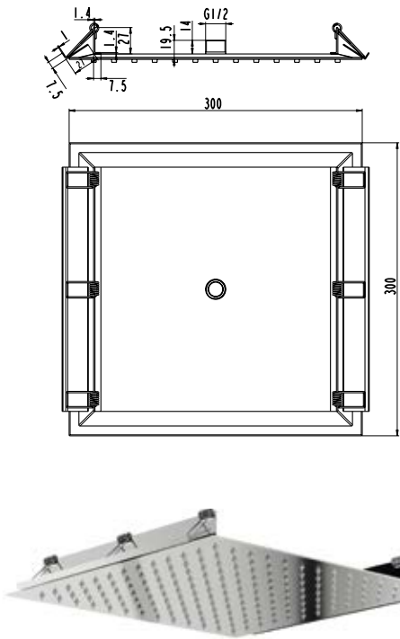
SHOWER HEAD SQUARE 30x30 cm Material: Stainless Steel (SS304)
