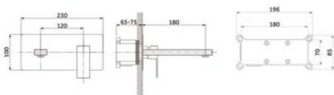
Ref. 3028 Wall-mounted basin mixer ORION CHROME
